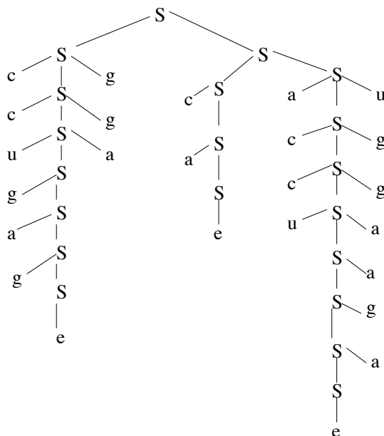
Figure 2: Parse tree for an example RNA structure. In the figure, “e” denotes the empty string \varepsilon .
